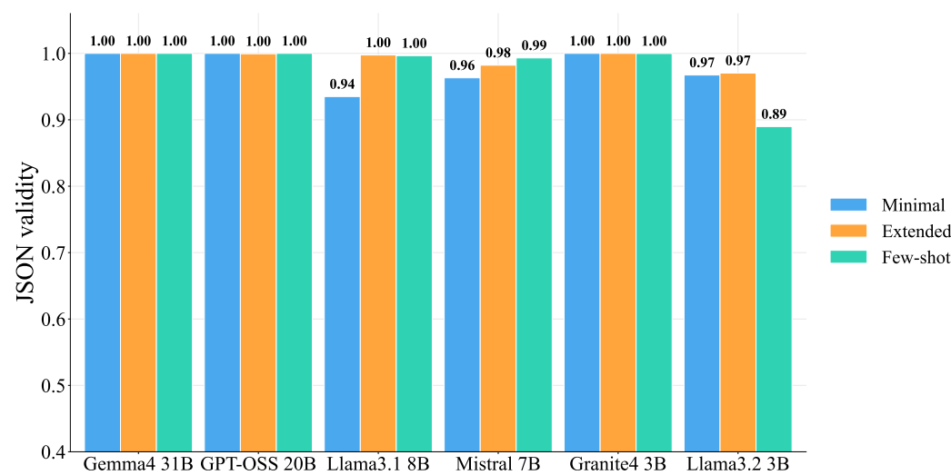
Figure 2. JSON validity by model and prompting regime (bars: minimal, extended, few-shot). Across almost all configurations the models emit parseable JSON at or near the ceiling (with Llama 3.2 3B under few-shot as an exception due to preamble wrapping); the residual small-model deficits under weaker prompts are predominantly schema violations rather than malformed JSON (cf. the schema-validity column of Table 4).
